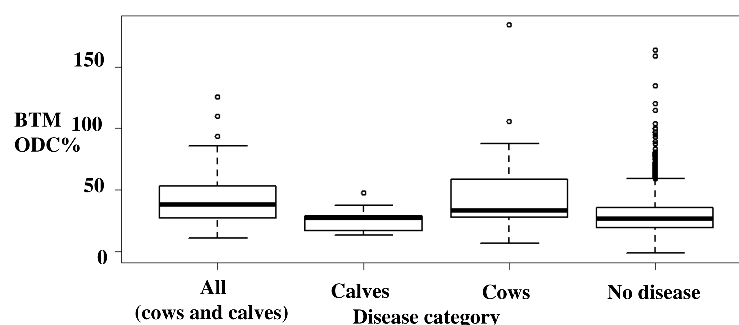
Fig. 2 Bulk tank milk (BTM) antibody levels (ODC%) in three categories of farmer reported primary clinical signs in Mycoplasma bovis outbreak or no reported outbreak
